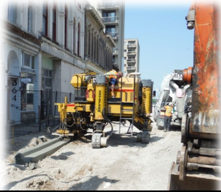
Example of curb machine placing curb in last Phase of Talbot Construction
